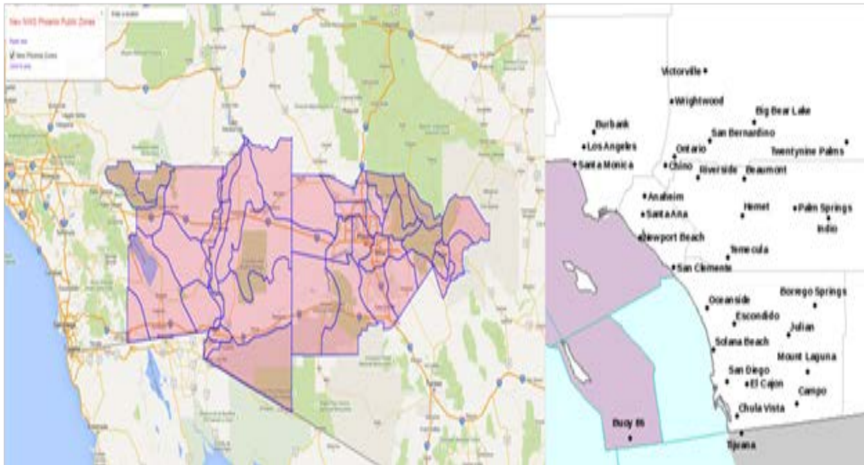
Fig C-1: Illustrates the public zones serviced by the National Weather Service Office in Phoenix and San Diego. Imperial County, including southeast sections of Riverside County are part of the reporting public zone areas from the Phoenix office
